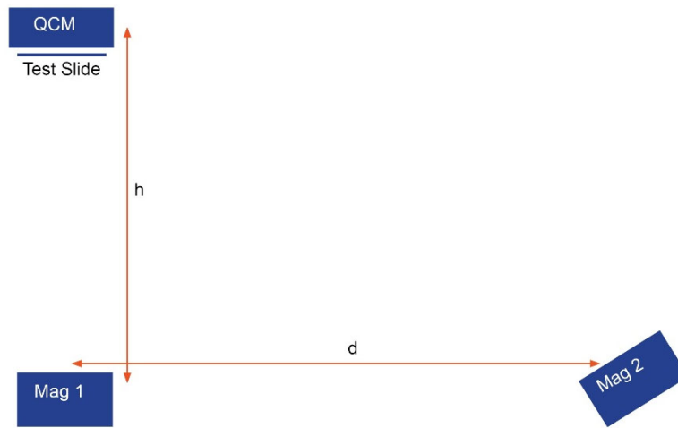
Figure 1. Side schematic of Experimental setup 1. Two magnetrons are mounted in a plane h=30 cm below a horizontal glass slide and quartz crystal monitor (QCM) sensor. The second magnetron, labeled "Mag2", is a distance d=40 cm from the first magnetron (labeled "Mag1").
