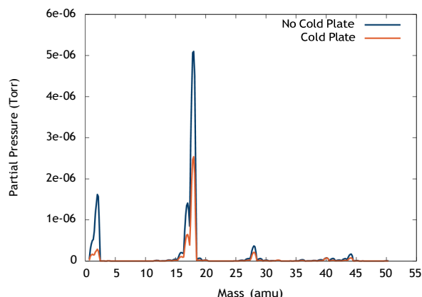
Figure 3. Two example Residual Gas Analyzer (RGA) scans, with (orange) and without (blue) the \text{LN}_2 cold plate operating. The most prominent peak in both scans, \text{H}_2\text{O}^+ ions at 18 amu, decreases by a factor of two when the cold plate is below -140^\circ\text{C} .
