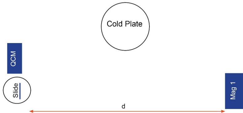
Figure 2. Overhead schematic of Experimental setup 2. A single magnetron is mounted horizontally in the chamber, d=72.4 cm from a test slide. The test slide is affixed upright to a small rotation stage to allow for angular rotation of the test slide with respect to the sputtering source. A 180 mm diameter LN 2 cold plate mounted below the plane of the magnetron and test slide provides additional water vapor pumping. The quartz crystal monitor (QCM) sensor is mounting next to the test slide, at the same source to substrate distance as the test slide.
